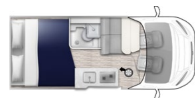
E-Van 6 XL Premium \rightarrow 5990 mm
