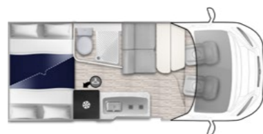
E-Van DUO Trend \rightarrow 6360 mm
